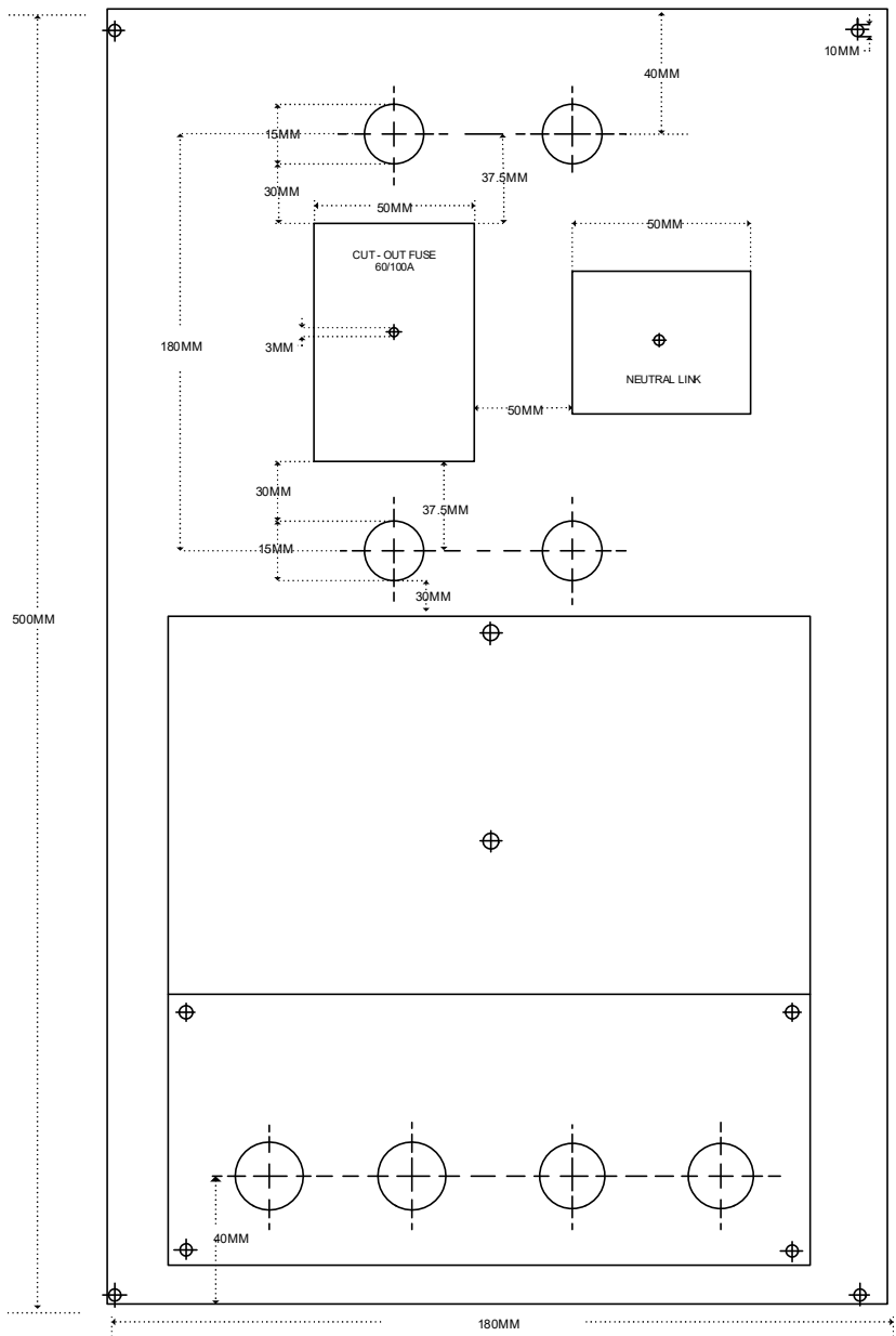
DRAWING NO 3B : SINGLE PHASE METERING ARRANGEMENT
