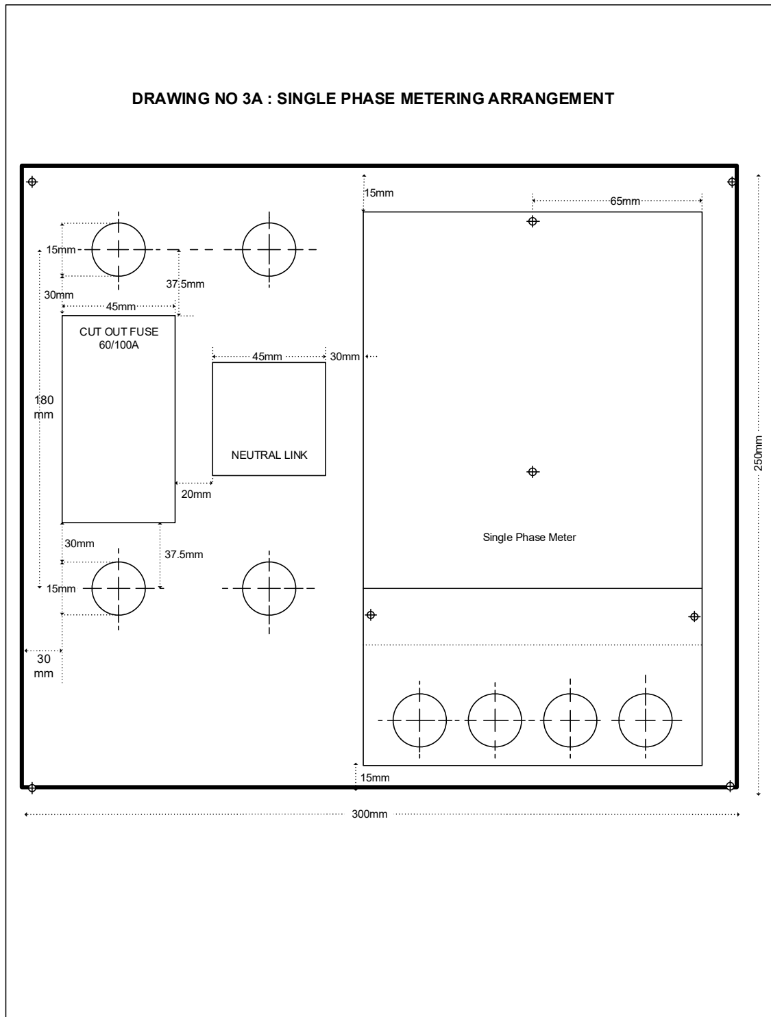
DRAWING NO. 3A: SINGLE PHASE METERING ARRANGEMENT
