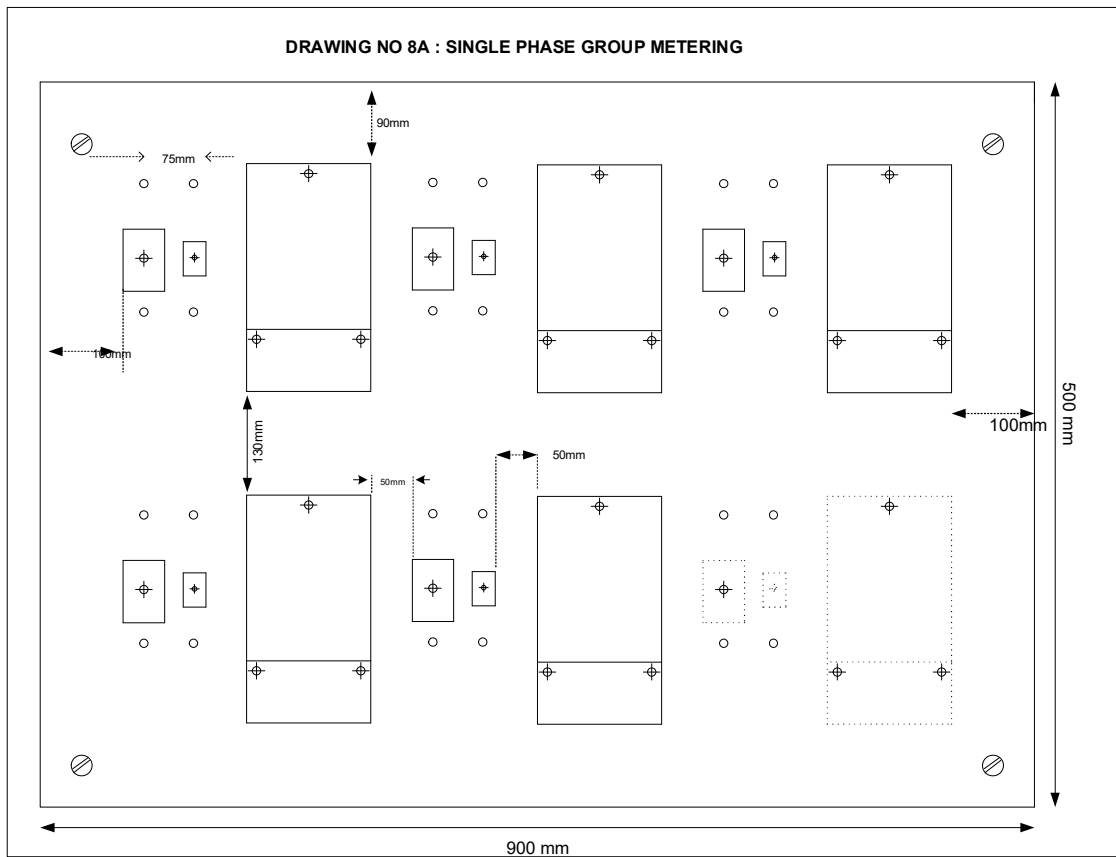
DRAWING NO. 8A: SINGLE PHASE GROUP METERING
