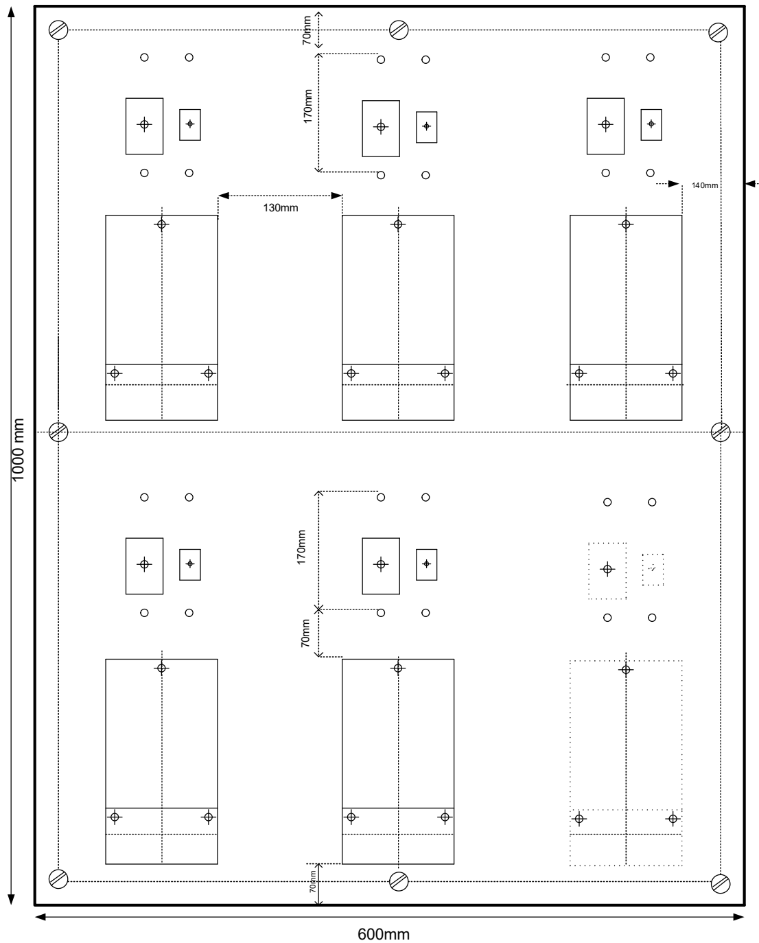
DRAWING NO 8B : SINGLE PHASE GROUP METERING
