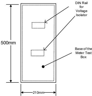
Drawing 11P - Side View
