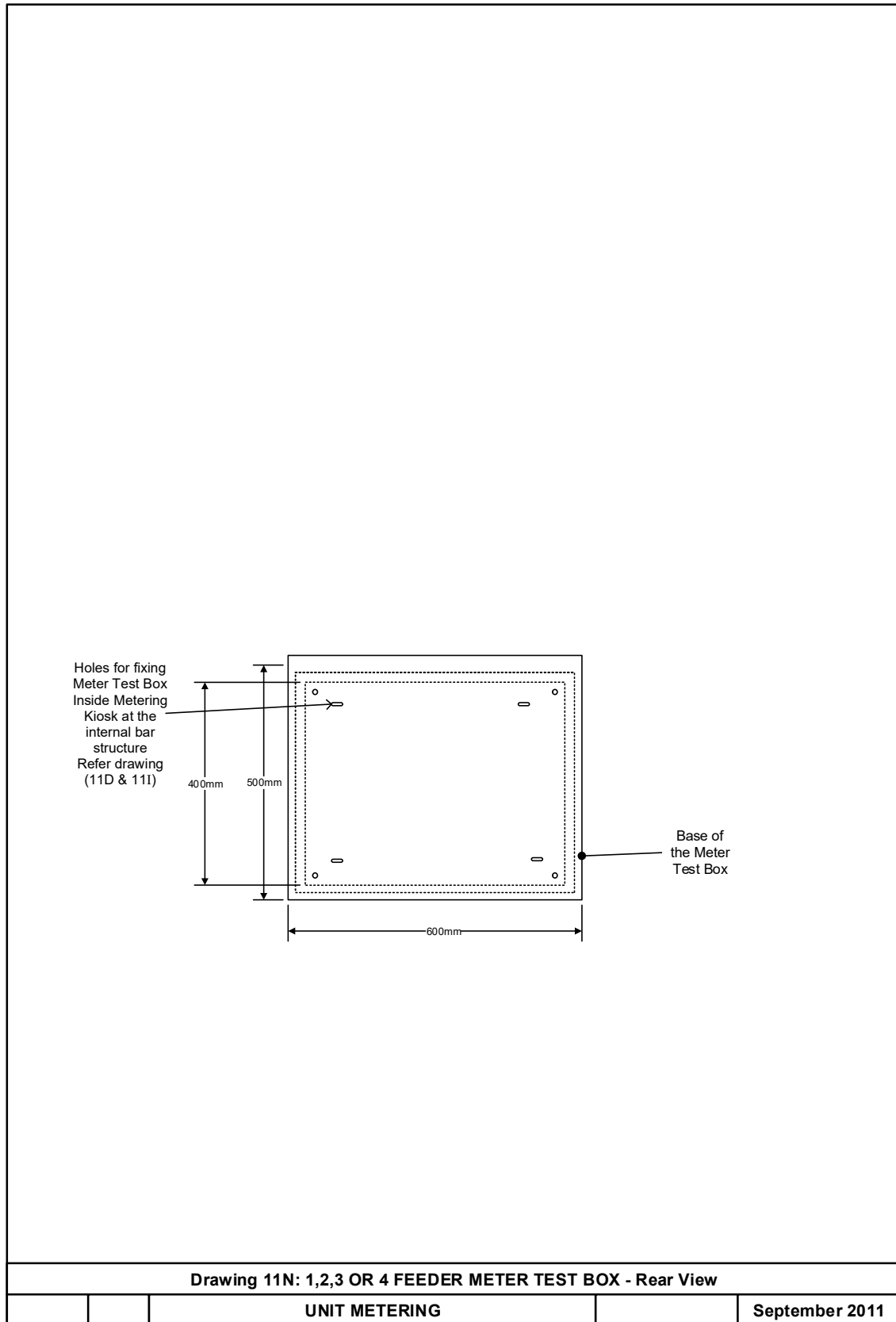
DRAWING 11N: MV/HV, 1, 2, 3 OR 4 FEEDER METER TEST BOX – REAR VIEW
