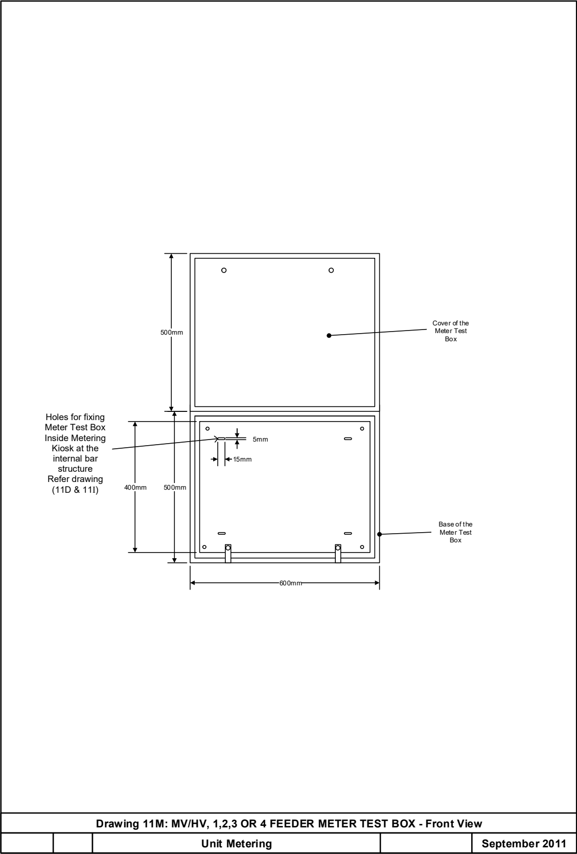
DRAWING 11M: MV/HV, 1, 2, 3 OR 4 FEEDER METER TEST BOX – FRONT VIEW
