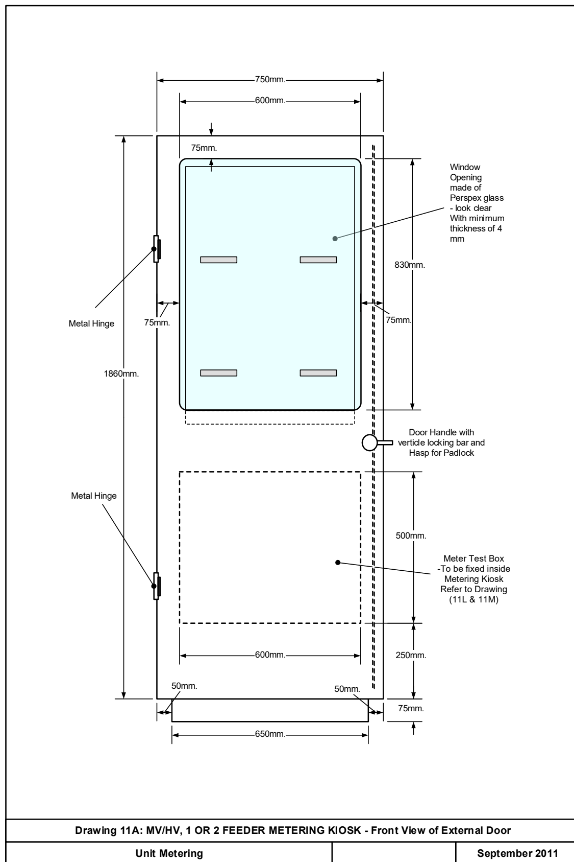
DRAWING 11A: MV/HV, 1 OR 2 FEEDER METERING KIOSK (FRONT VIEW OF EXTERNAL DOOR)
