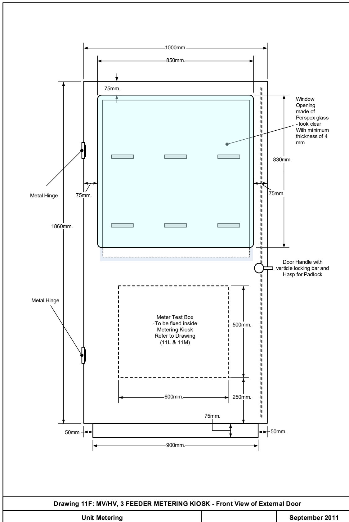
DRAWING 11F: MV/HV, 3 FEEDER METERING KIOSK (FRONT VIEW OF EXTERNAL DOOR)
