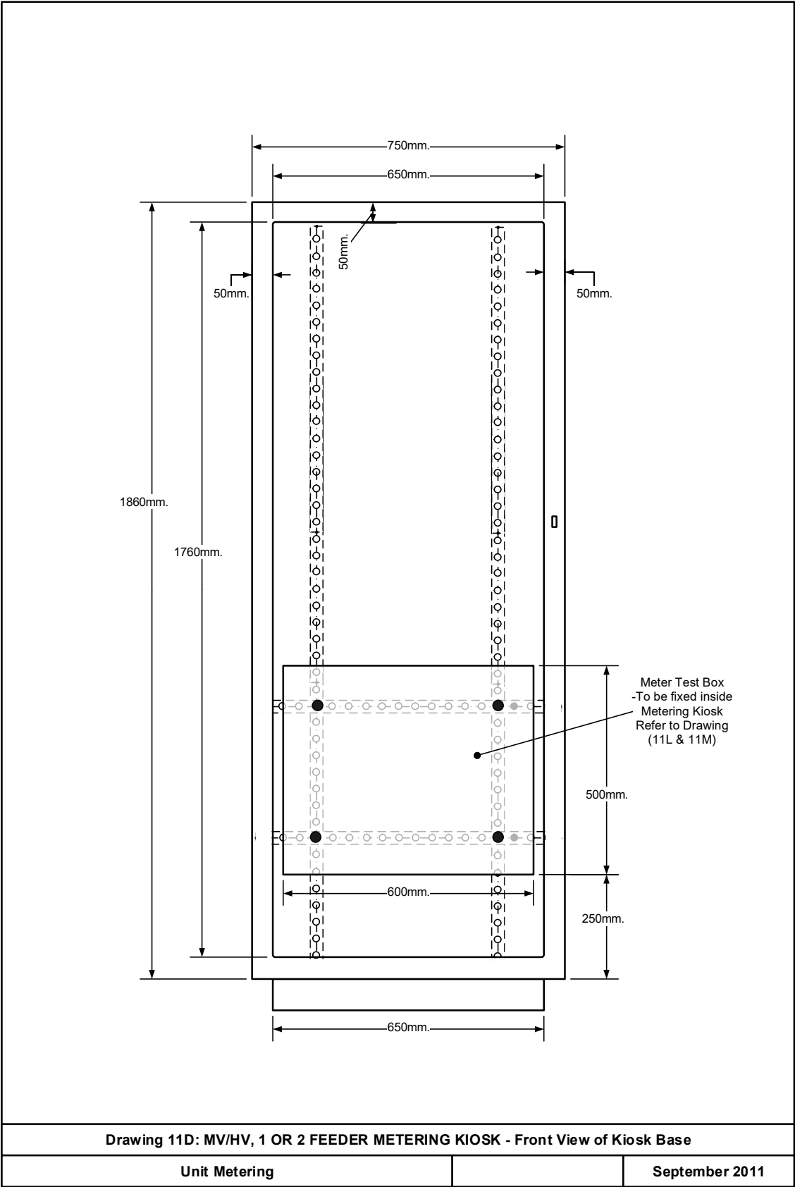
DRAWING 11D: MV/HV, 1 OR 2 FEEDER METERING KIOSK (FRONT VIEW OF KIOSK BASE)
