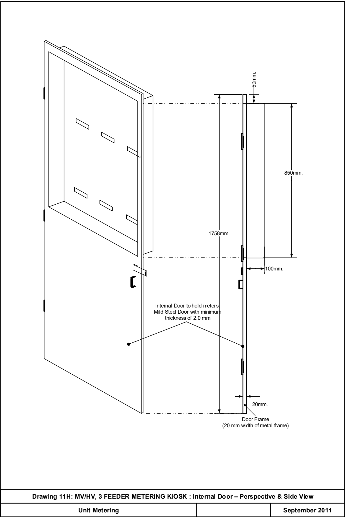
DRAWING 11H: MV/HV, 3 FEEDER METERING KIOSK (INTERNAL DOOR – PERSPECTIVE AND SIDE VIEW)
