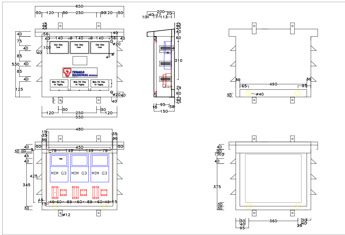
DRAWING NO. 1C (I) - SINGLE PHASE METER PANEL (POLE)
