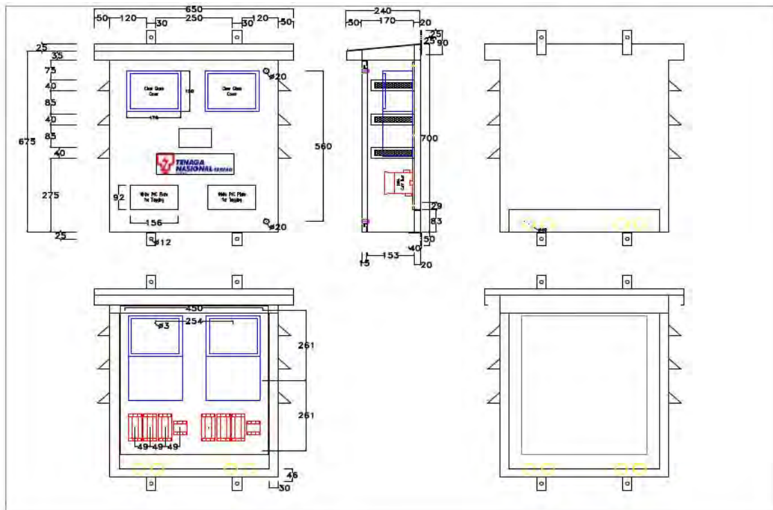
DRAWING NO. 1C (II) - THREE PHASE METER PANEL (POLE)
